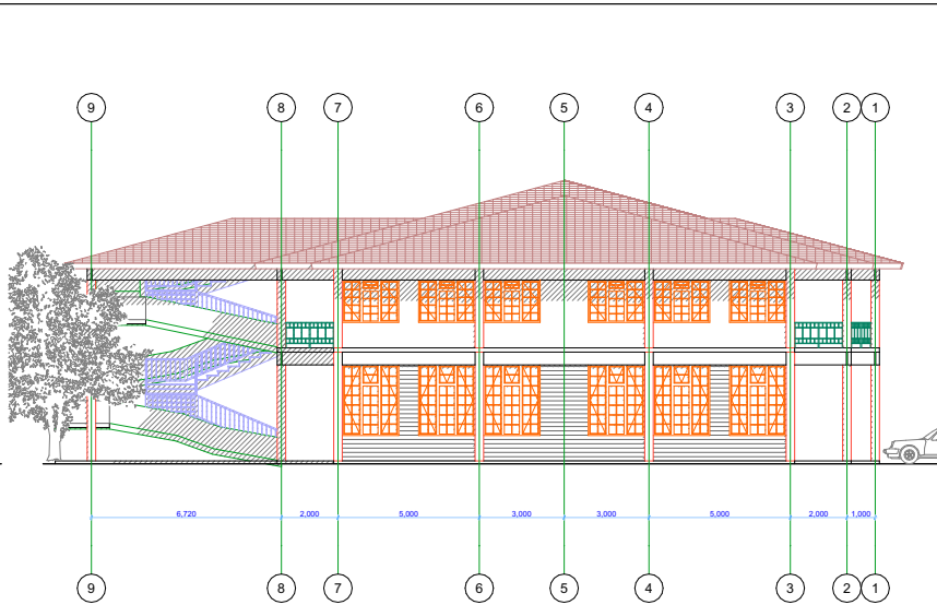
West Elevation
