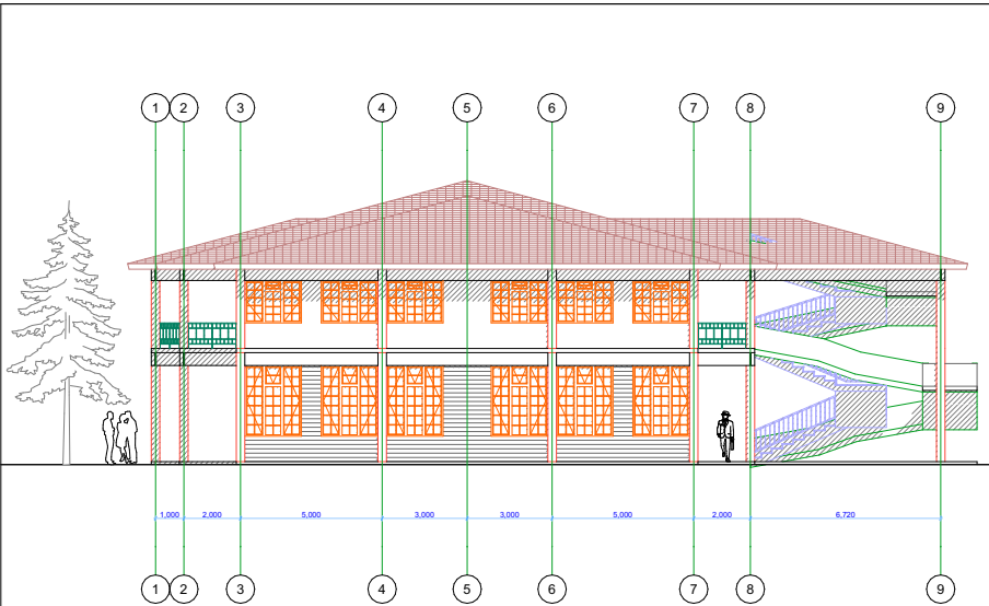
East Elevation
